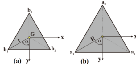
Fig. 2. Moving platform and upper platform.
