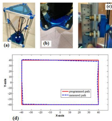
Fig. 6. a) construction of parallel robot, b) the method to verify the position of end-effector in x-axis and y-axis, c) the method to verify the position of mobile platform in z-axis, d) the verification result on the accuracy of robot in following the programmed trajectory.
