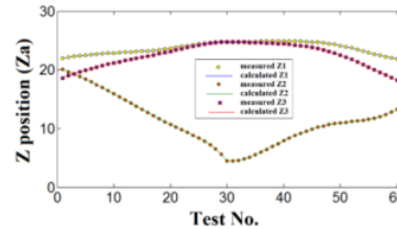
Fig. 5. Model verification using Siemens-NX.
